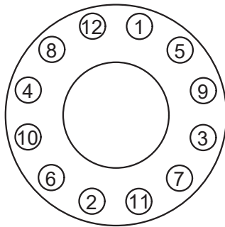
12-bolt
