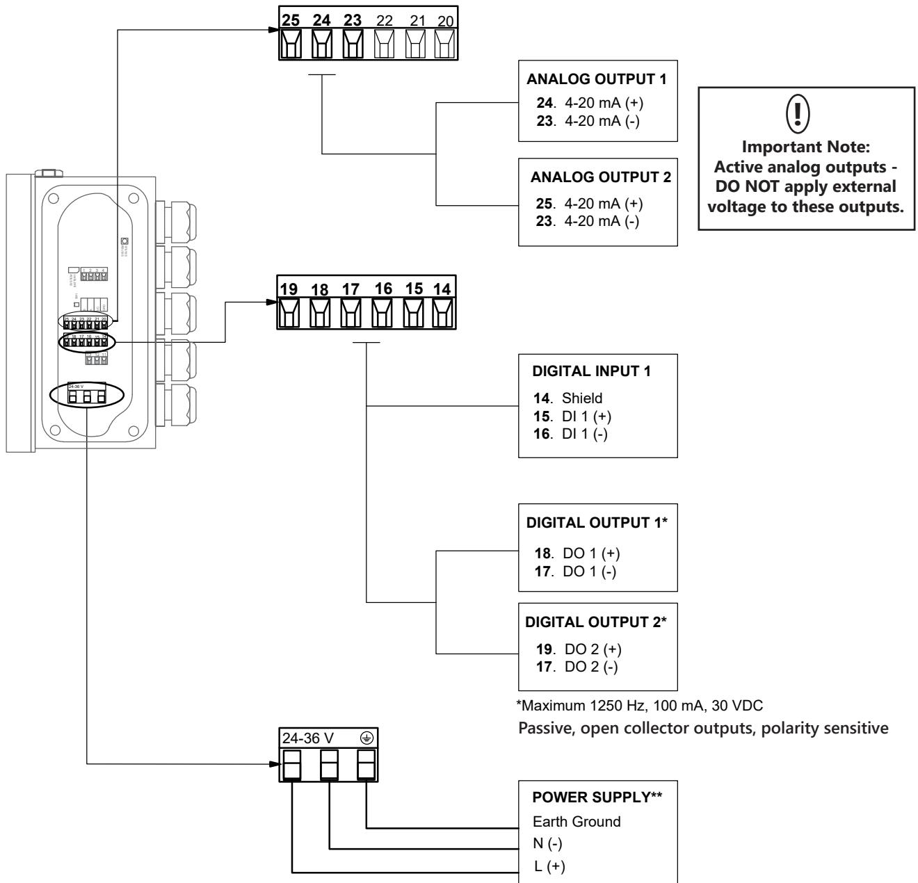
DIGITAL OUTPUT SCHEMATIC
