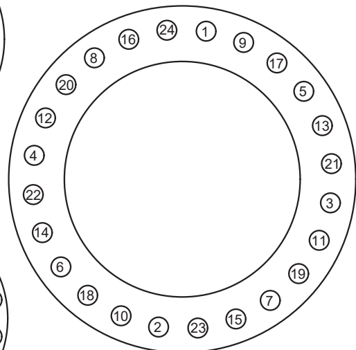
24-bolt
