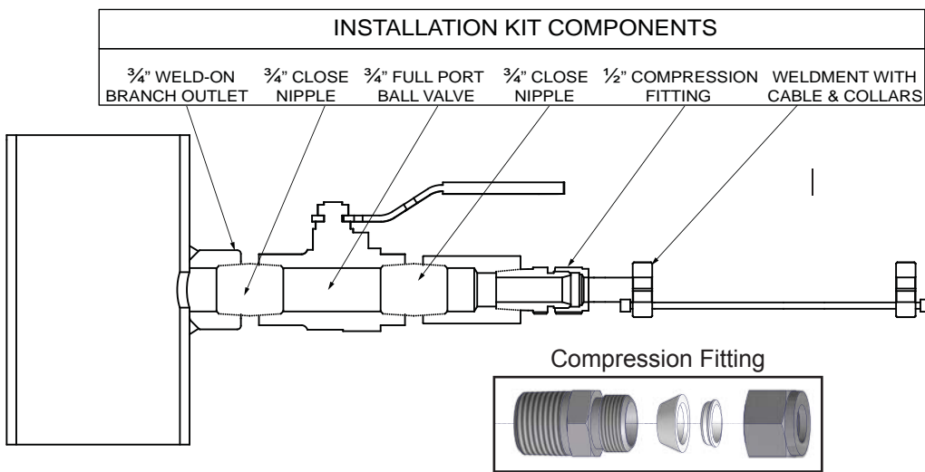
(Exploded view)
